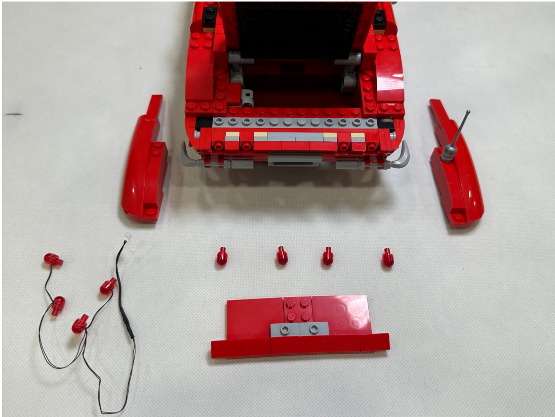
Start assembling the rear light, remove the shown parts first
