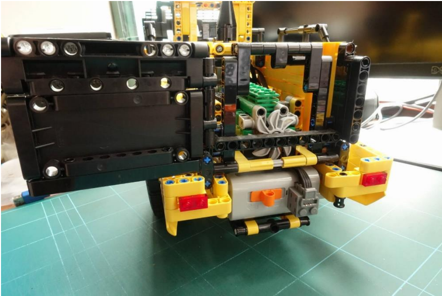
Connect the 4-stud plug of the light kit to the battery box
