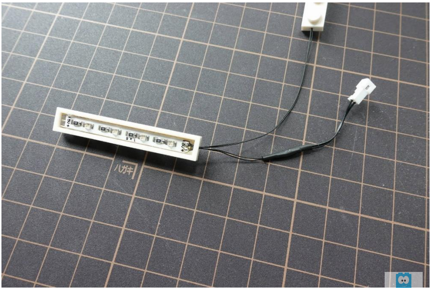
Install the A lights
