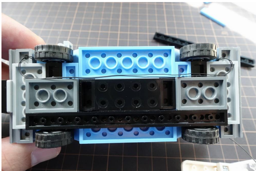
Fix the wire under black plate
