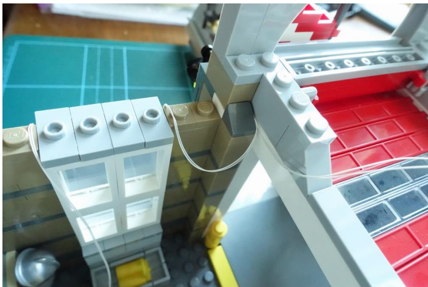
Install the left wall light
